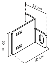
Lower Bracket
